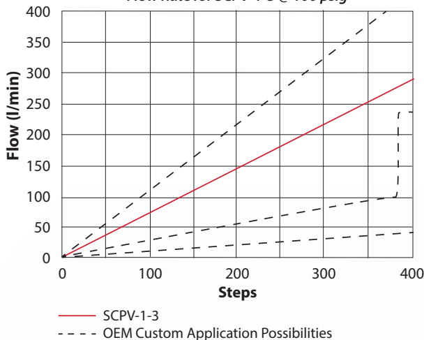
Characteristic Curve Flow Rate for SCPV-1-3 @ 100 psig
